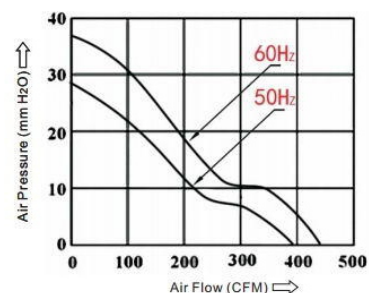
P&amp;Q CURVE (at Rated Voltage)
