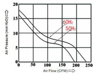
P&amp;Q CURVE (at Rated Voltage)
